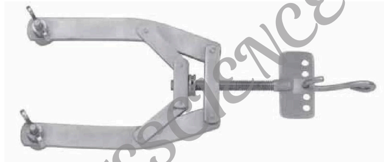
K WIRE TRACTOR SMALL/MEDIUM/LARGE
